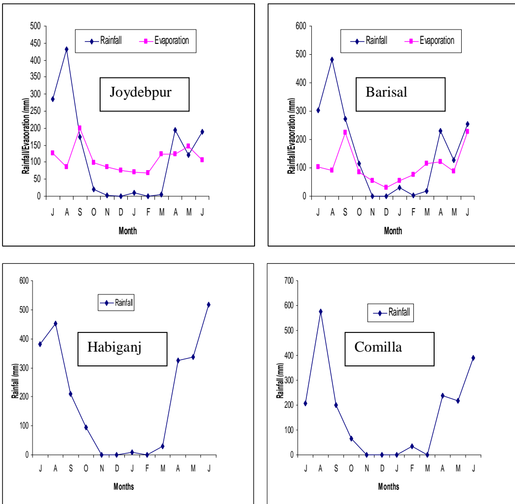
Fig. 2: Monthly total rainfall (mm) and evaporation (mm) of Gazipur and other three regional stations, July 2011 to June 2012.
